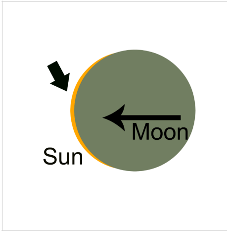
2nd contact
