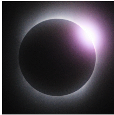
diamond ring
