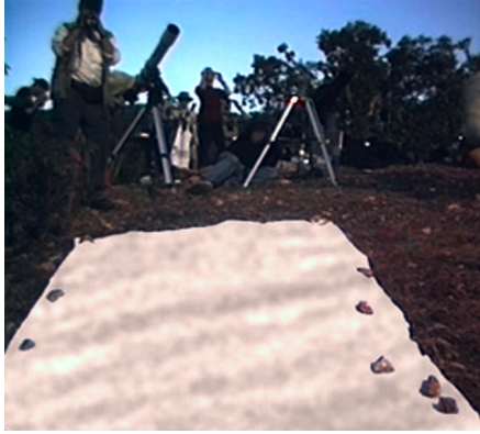
shadow bands
