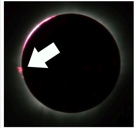
Baily's beads
