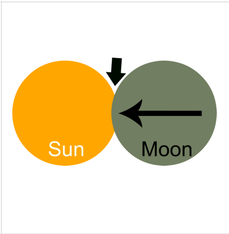
1st contact
