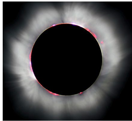
totality
