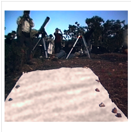
shadow bands
