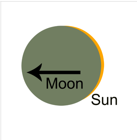
3rd contact
