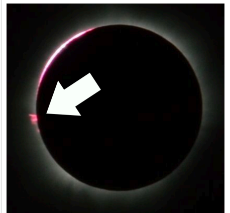
Baily's beads
